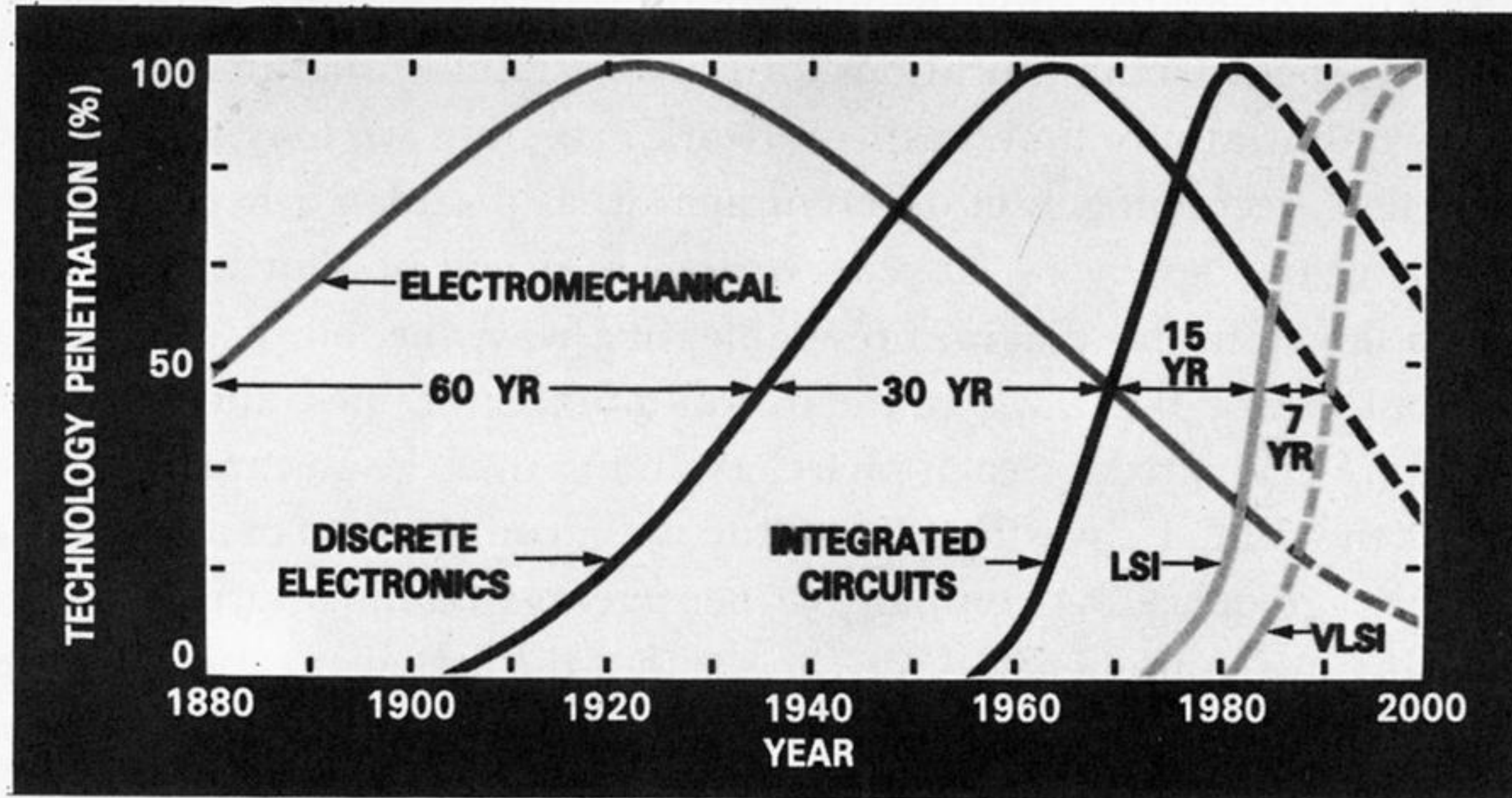
FIGURE 5. Component technology evolution. (After J. M. Connell, Spring Comcon 1981 (updated).)
